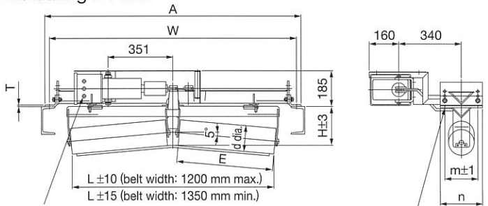
The above diagram illustrates the external dimensions of model HAB-MR-105052H (belt width: 1050 mm).
