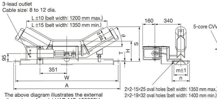
The above diagram illustrates the external dimensions of model HAB-MC-105302H (belt width: 1050 mm, trough angle: 30°).
